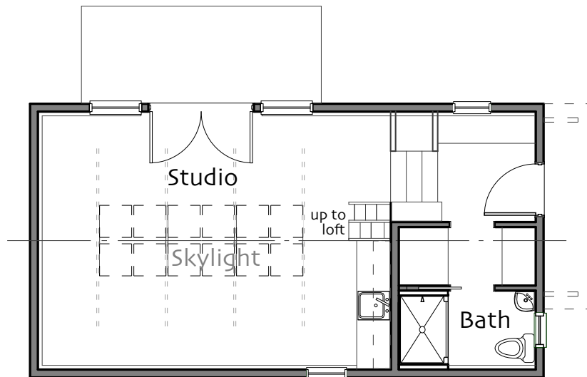
Floor Plan
